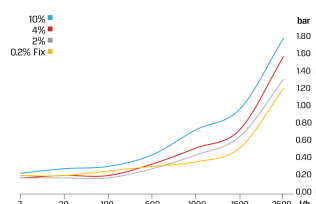
Pressure Loss
