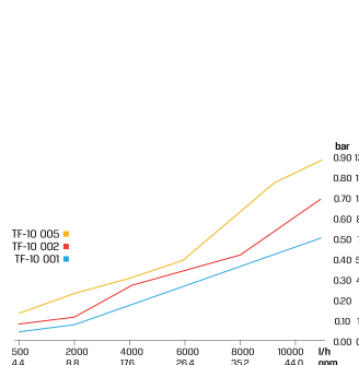
Pressure Loss
