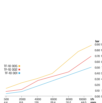
Pressure Loss
