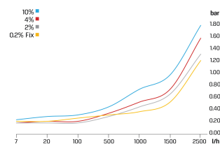
Pressure Loss
