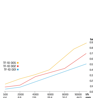
Pressure Loss
